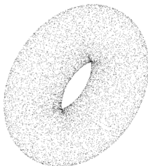
FIGURE 1.1 – Point cloud sampled from a torus.
