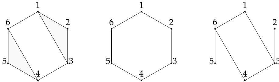
FIGURE 5.2 – The complex on the left has two different 1-cores, the one in the middle is obtained after removing the inner edges [1,3] and [4,6] , and the one in the right by removing the outer edges [1,2] and [4,5] . Note that the one in the right can be further strong collapsed.
