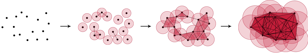
FIGURE 2.6 – A sequence of simplicial complexes connected through inclusions.
