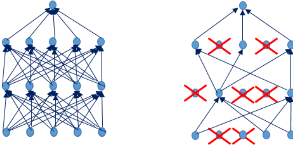
Figure A.1: Left: Normal neuronal network. Right: Neuronal network with dropout nodes. Figure adapted from [40].
