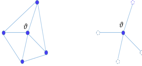
Figure 2.8: Left: The star of a vertex v (in the middle). Right: The open star of a vertex v (in the middle). Figure adapted from [38].
