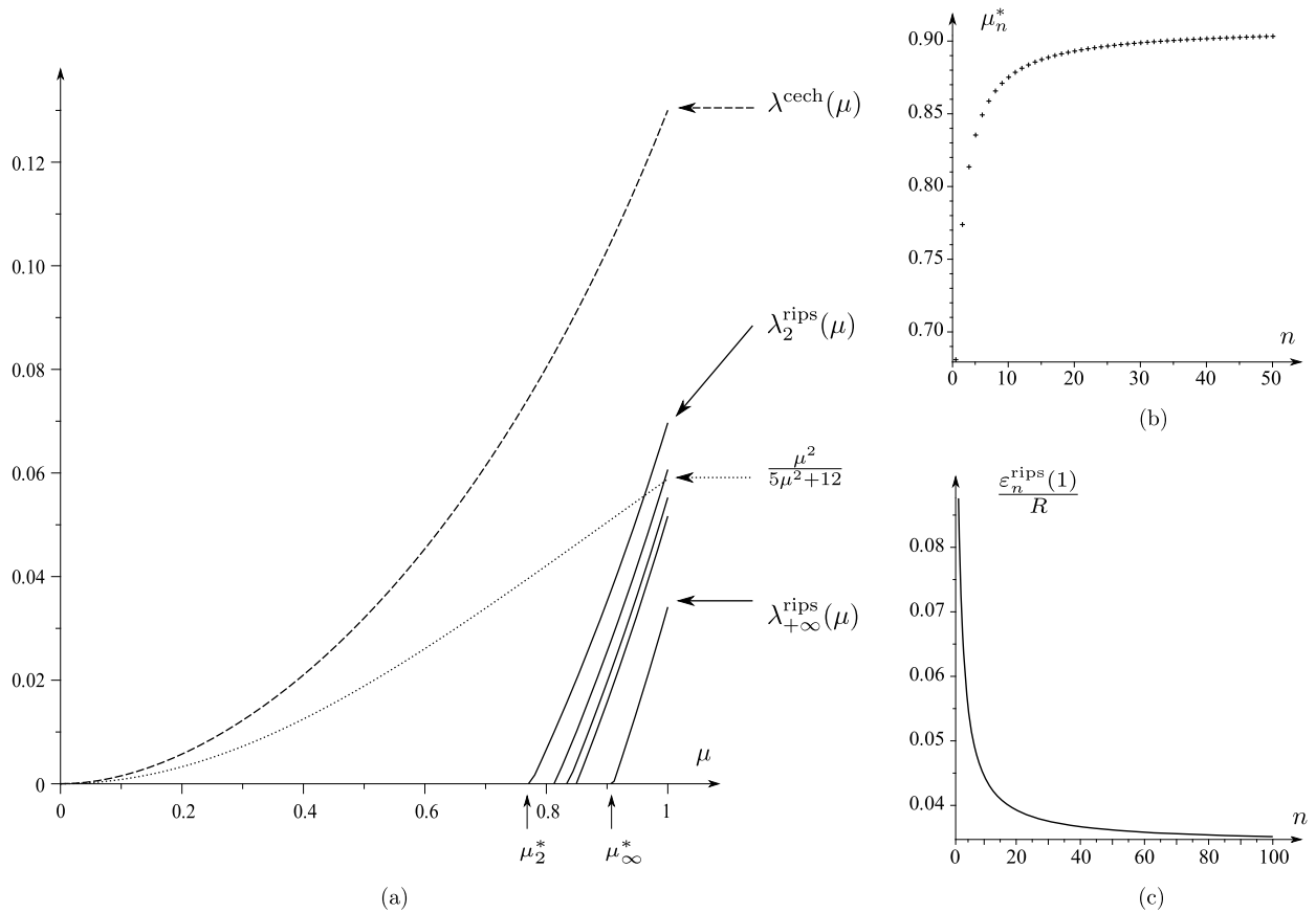
Fig. 9. (a) Best ratios \frac{\varepsilon}{R} we can get for a correct reconstruction of a shape with a positive \mu -reach either with the Čech or Rips complex for n \in \{2, 3, 4, 5, +\infty\} ; comparison with the ratio \frac{\mu^2}{5\mu^2+12} obtained in [16]. (b, c) \mu_n^* and \lambda_n^{\text{rips}}(1) as functions of n .
