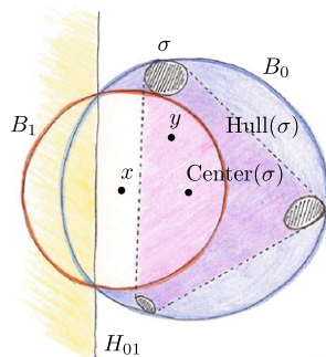
Fig. 3. Notation for the proof of Lemma 1.
