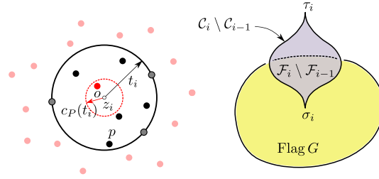
Fig. 6. Notation for the proof of Theorem 7. Left: \tau_i is the simplex whose vertices are points of P in B(z_i, t_i) . \sigma_i is the face obtained by keeping vertices on the boundary of B(z_i, t_i) . Right: Schematic representation of simplices in C_i \setminus C_{i-1} .
