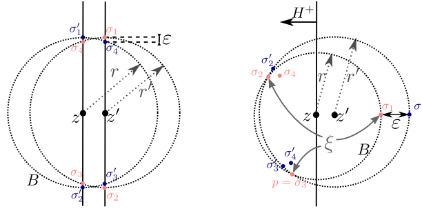
Fig. 11. Left: The bound on \|\text{Center}(\sigma) - \text{Center}(\sigma')\| in Lemma 16 is tight. Right: Notation for the proof of Lemma 16.
