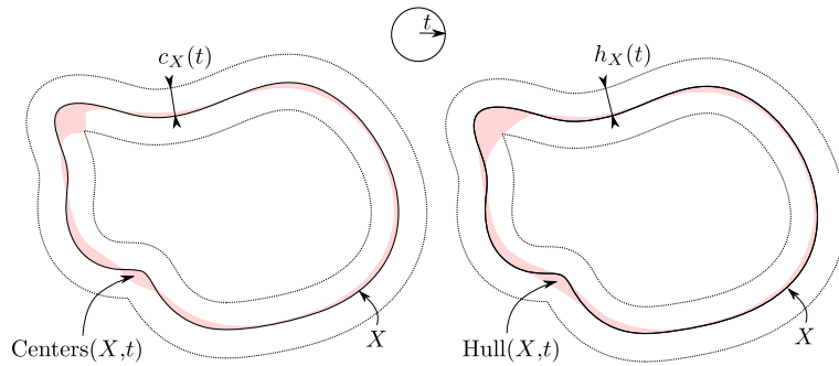
Fig. 2. Smallest offset of X containing \text{Centers}(X, t) on the left and \text{Hull}(X, t) on the right.
