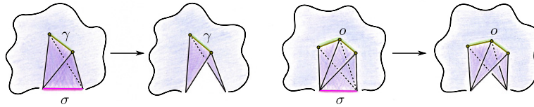
Fig. 5. Left: In a classical collapse, the link of \sigma has a unique inclusion-maximal simplex \gamma . Equivalently, the star of \sigma has a unique inclusion-maximal simplex \sigma \cup \gamma different from \sigma . Right: In an extended collapse, the link of \sigma is a cone with apex o .
