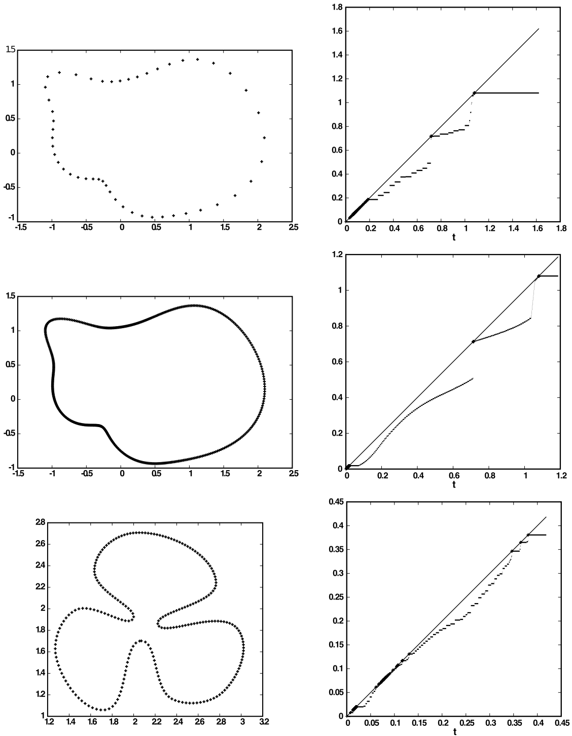
Fig. 10. Various point sets P on the left and corresponding convexity defects function c_P on the right.
