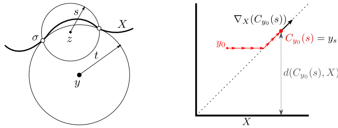
Fig. 8. Notation for the proofs of Lemma 11 on the left and Lemma 12 on the right.
