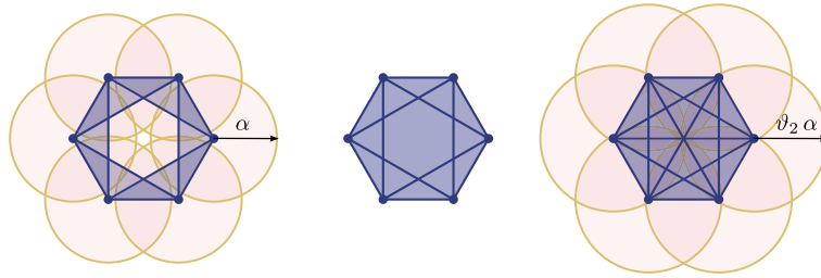
Fig. 1. Left: The Čech complex with parameter \alpha comprises six triangles and is homotopy equivalent to a circle. Middle: The Rips complex with parameter \alpha contains two more triangles and is homeomorphic to a 2-sphere. Its shadow is a topological disk. Right: The Čech complex with parameter \vartheta_2 \alpha contains all faces of the 5-simplex and is homeomorphic to a 5-ball.
