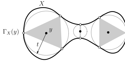
Fig. 4. The black points are the critical points of the curve X .
