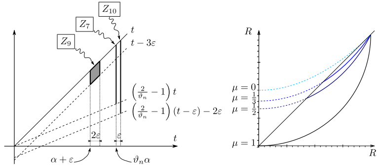
Fig. 7. Left: For i \in \{7, 9, 10\} , the hypotheses of Theorem i are depicted as regions Z_i avoided by the graph of a convexity defects function. Specifically, if c_P \cap Z_7 = \emptyset , Theorem 7 implies \mathcal{R}(P, \alpha) \simeq P^\alpha . If h_X \cap Z_9 = \emptyset , Theorem 9 implies \mathcal{C}(P, \alpha) \simeq X^{\alpha-2\epsilon} . If h_X \cap Z_{10} = \emptyset , Theorem 10 implies \mathcal{R}(P, \alpha) \simeq X^{2\alpha-\vartheta_n\alpha-2\epsilon} . Right: Upper bound on h_X for \mu \in [0, \frac{1}{3}, \frac{1}{2}, 1] provided by Lemma 12.
