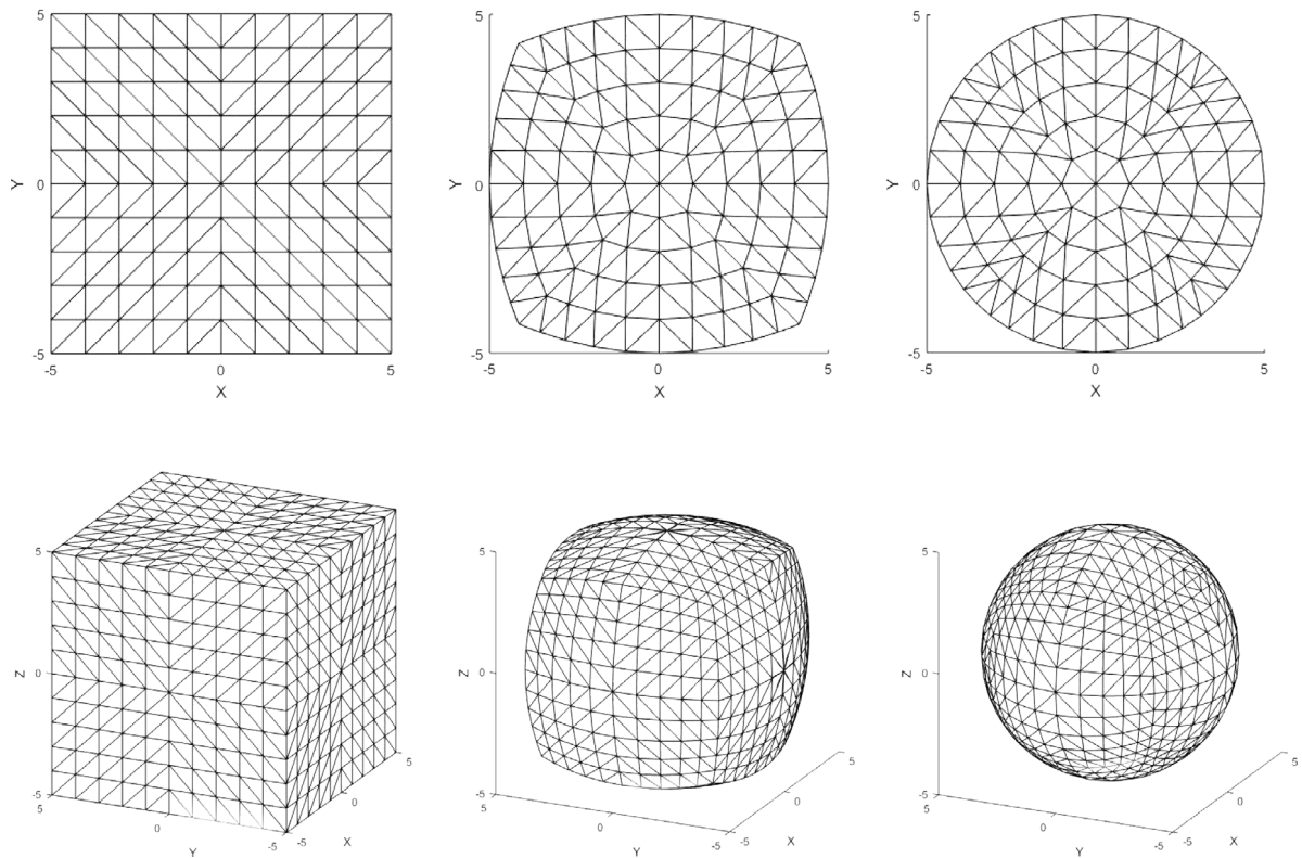
Fig. 1. The images of the standard triangulation in \mathbb{R}^2 (upper row) and \mathbb{R}^3 (lower row) restricted to [-5, 5]^2 and [-5, 5]^3 and the same restrictions under the mappings \mathbf{H}_0^1 = \text{Id}_{\mathbb{R}^n} , \mathbf{H}_{1/2}^1 , and \mathbf{H}_1^1 = \Phi from left to right ( \rho(x) = 1 ), see Definition 2.10 for \mathbf{H}_i^1 .
