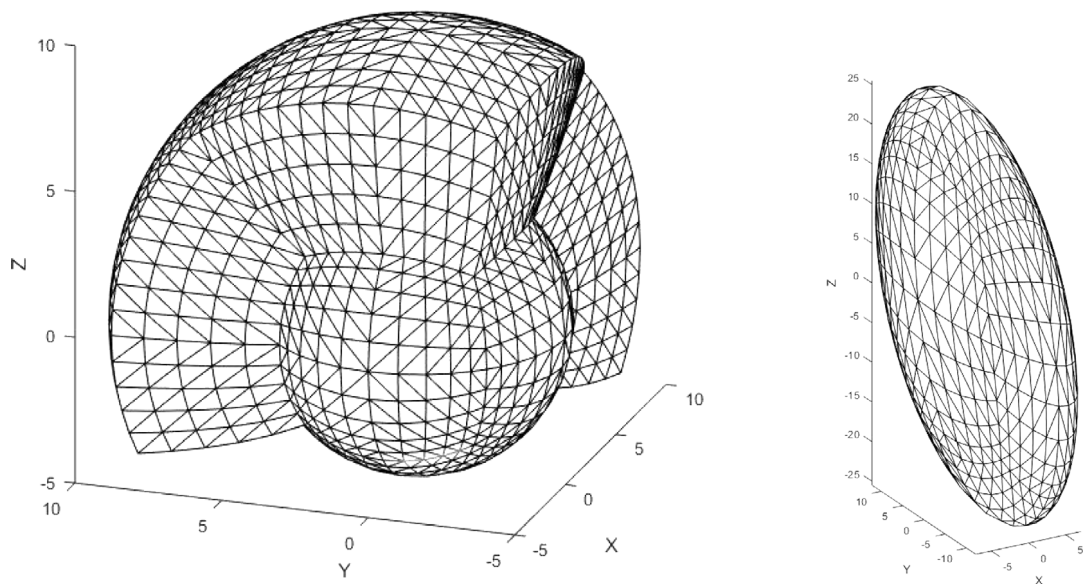
Fig. 2. Left: The image of the restriction of the standard triangulation in \mathbb{R}^3 to [-5, 10]^3 under the mapping \mathbf{H}_1^1 = \Phi . Right: The image of the restriction of the standard triangulation in \mathbb{R}^3 to [-5, 5]^3 under the mapping \mathbf{x} \mapsto A\Phi(\mathbf{x}) with the matrix A = ((1, -1, 0)^T, (-1, 2, 1)^T, (0, 1, 5)^T) .
