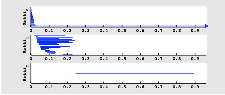
FIGURE 8. Persistence barcode for \mathbf{Del}(A, B) with A \subset B sampled from X = S^2 ; |A| = 20 , |B| = 400 .
