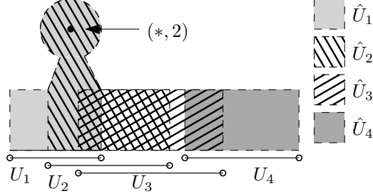
Figure 6: Construction of \{\hat{U}_i\} from \{U_i\} assuming \vartheta = \{U_1, U_2\} .
