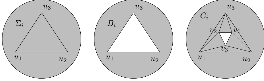
Figure 1: The complexes \Sigma_i , B_i and C_i
