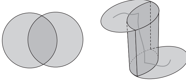
Figure 7: Left: a cover \{U_1, U_2\} consisting of two sets. Right: the space \Delta(\{U_1, U_2\}) , and a gray path from the proof of Lemma A.8.
