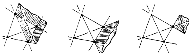
Figure 7.1: Regions P_I of a 3-simplex, with |I| = 1 to the left, |I| = 2 in the middle, and |I| = 3 to the right.
