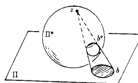
Figure 6.2: Under inversion, the image of a hyperplane is a d -sphere, and every (d-1) -sphere in the hyperplane maps to a (d-1) -sphere on the d -sphere.
