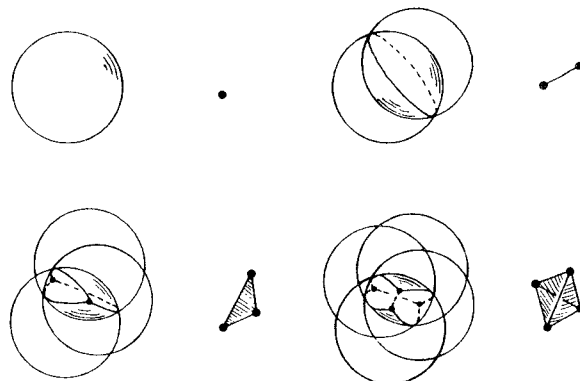
Figure 6.1: The intersection of one, two, three, and four 3-balls. The face structure is dual to that of a vertex, an edge, a triangle, and a tetrahedron.
