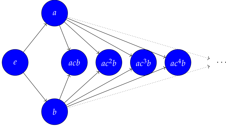
Figure 5.3: Graphical illustration of a monoid that is not good. The monoid is the non-commutative monoid generated by three elements a, b, c modulo the congruence generated by ac^n b \approx bc^n a for all n \in \mathbb{N}_{>0} . The plcm of \{a, b\} are the elements of the countable set \{ac^n b\}_{n \in \mathbb{N}_{>0}} .
