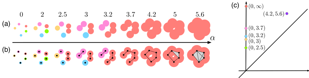
Figure 3.2: Computing persistent homology of a point cloud in \mathbb{R}^2 . (a) The union-of-balls filtration with respect to a certain sequence of increasing parameter values. (b) The Čech filtration of (a). (c) Persistence diagrams of 0-dimensional and 1-dimensional homology combined.
