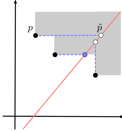
Figure 3.5: The three black points mark the three critical points of some simplex \sigma in X . The shaded area denotes the positions at which \sigma is present in the bifiltration. Along the given slice (red line), the dashed lines denote the first position where the corresponding critical point “affects” the slice. This position is either the upper-vertical, or right-horizontal projection of the critical point onto the slice, depending on whether the critical point is below or above the line. For \sigma , we see that it enters the slice at the position marked by the blue point.
