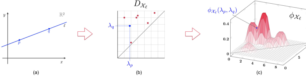
Figure 6.1: An illustration of the construction of a feature map for multiparameter persistence. (a) Given a bifiltration \mathcal{X} and a point (p, q) \in \Delta^{(2)} , the line \ell passing through them is depicted and the parameter \lambda_p and \lambda_q computed. (b) The point (\lambda_p, \lambda_q) is embedded in the persistence diagram of the monofiltration \mathcal{X}_\ell obtained as the slice of \mathcal{X} along \ell . (c) The point (\lambda_p, \lambda_q) is assigned the value \phi_{\mathcal{X}_\ell}(\lambda_p, \lambda_q) via the feature map \phi .
