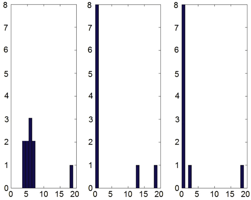
Fig. 3. (a) (resp. (b), (c)) The histogram of the lengths of the barcode B1 (resp. B2, B3 ) shown in Fig. 2.
