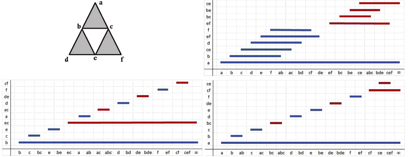
Fig. 2. An example of three different persistence barcodes obtained from the same simplicial complex. Intervals corresponding to 0-barcode are in blue. Intervals corresponding to 1-barcode are in red. Top-right: barcode B1 ; down-left: barcode B2 ; down-right: barcode B3 . The filters can be read on the x-axis of each of the diagrams. For B1 , it is F1 = \{a, b, c, d, e, f, ab, ac, bd, cf, de, ef, bc, be, ce, abc, bde, cef\} ; For B2 , F2 = \{b, c, bc, e, be, ec, a, ab, ac, abc, d, bd, de, bde, f, ef, cf, cef\} ; For B3 , F3 = \{a, b, ab, c, ac, bc, abc, d, bd, e, de, bde, f, ef, cf, ce, cef\} . (For interpretation of the references to color in this figure caption, the reader is referred to the web version of this article.)
