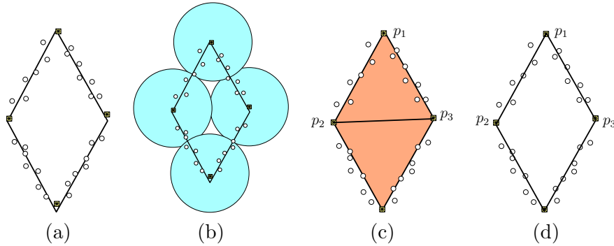
Figure 2: (a) A set of points P sampling a curve. The four square points are subsampled landmarks Q . (b) The union of balls around subsamples in Q for some radius r . Its corresponding Rips complex is shown in (c), containing two triangles. Shrinking the radius r however will disconnect points p_1 and p_3 . The witness complex, shown in (d), has the same topology as the hidden curve. For this particular example, the graph induced complex is the same as (d).
