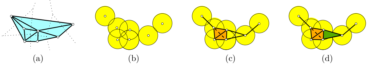
Figure 1: (a) Delaunay complex (solid lines). Dotted lines represent the dual Voronoi diagram. (b) The union of balls around the same set of points for a specific radius r . The Čech complex is in (c) while the Rips complex is in (d). Note that both the Čech and Rips complex contain the tetrahedron in the middle. The Rips complex contains the triangle on the right, while the Čech complex does not, as the three corresponding balls do not have common intersection.
