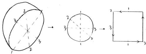
Figure 4.10: Reduction of \mathbb{R}P^2 [8].
