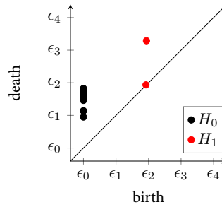
Figure 6.3: Persistence diagram of the Vietoris–Rips filtration shown in Figure 6.2. Here, we overlay the birth ( x -axis) and death ( y -axis) events of topological features for connected components (corresponding to the Betti number \beta_0 and the homology group H_0 ) as black dots, and cycles (corresponding to the Betti number \beta_1 and the homology group H_1 ) as red dots.
