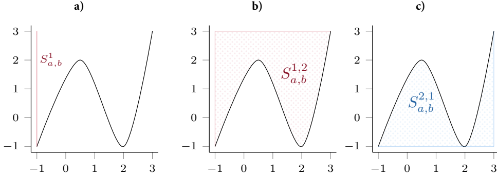
Figure 5.1: Visualisation of the signature for the first and second order terms. First-order terms are of the form S_{a,b}^i and represent the increment of a path along dimension i . Second-order terms of the form S_{a,b}^{i,j} and for i \neq j correspond to signed areas above or below a path and are related to the Lévy area, i.e., the signed area between the path (evaluated from a to b ) and the chord (or linear interpolation) of X_a and X_b .
