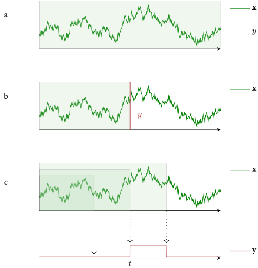
Figure 2.1: Illustration of three types of time series classification tasks. Time-varying variables are written as vectors in bold. Panel a: Whole series classification. The time series values \mathbf{x} are provided with a label \mathbf{y} . Panel b: Window-based classification. The time series values \mathbf{x} are provided with a time-stamped label \mathbf{y} (red). Panel c: Per-timepoint classification. Both the input time series \mathbf{x} and the labels \mathbf{y} are sequences. Three predictions are highlighted where all data up until the given point in time is used for prediction. The filled boxes (green) indicate which windows of time series data are used for prediction.
