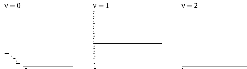
Figure 4: Betti 1 persistence intervals of witness complexes for the Mumford data: varying v , and keeping fixed K = 125 , cut = 25%, 50 vertices, intrinsic graph metric (with k = 125 ).
