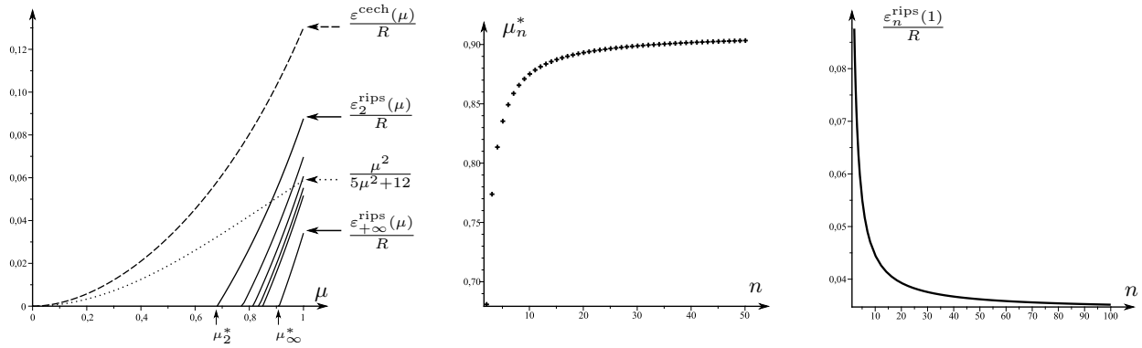
Figure 8: Left: Best ratios \frac{\varepsilon}{R} we can get for a correct reconstruction of a shape with a positive \mu -reach either with the Čech complex or the Rips complex for n \in \{2, 3, 4, 5, 6, +\infty\} ; comparison with the ratio obtained in [15]. Middle: \mu_n^* as a function of n . Right: \frac{\varepsilon_n^{\text{rips}}(1)}{R} as a function of n .
