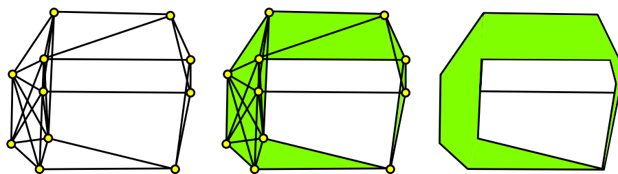
Fig. 1 A connectivity graph in the plane ( left ) determines a five-dimensional (Victoris-)Rips complex ( center ) and its two-dimensional projected shadow ( right )
