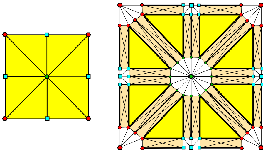
Fig. 7 A 3-colored simplicial complex K and its blowup \tilde{K} , whose flag completion is homotopy equivalent to K . Opposite edges of K (and thus \tilde{K} ) can be identified to yield a torus, projective plane, or Klein bottle
