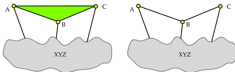
Fig. 4 ACXY (left), or ABCX (right), splits into two cycles in the presence of [BX] , [BY] , or [BZ]
